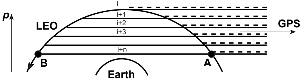
Figure 3.6: Visualisation of the onion peeling method (modified version of a figure taken from Syndergaard (2007)). Calibrated TEC values, \widetilde{TEC} , are calculated by \widetilde{TEC} = solid – dashed lines.
