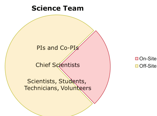
Fig. 5.2: Typical composition of a science team
