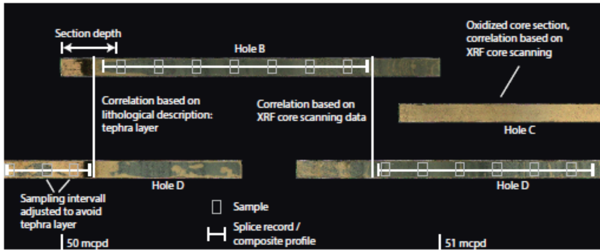
Fig. 4: The CORELYZER tool as implemented through the Lamont-Doherty Earth Observatory (LDEO) allows core correlation on data obtained in adjacent Holes B and D. In the case of Lake Obriid, core correlation was performed using lithological information (tephra layer/volcano-stratigraphy) and information derived from correlating high-resolution XRF scanning data loaded into the CORRELATOR software package. Marked are the “splice record” and the “samples”, which were taken from the splice record on a regular interval. Special care ought to be taken regarding the various depth scales involved.
