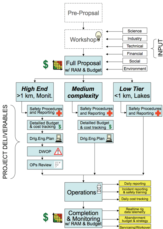
Fig. 2.9: Risk management for ICDP projects; see text for detailed description. (RAM: risk assessment matrix; DWOP: drilling well on paper; OPs review: post drilling operational review)
