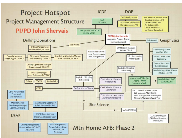
Fig. 2.7: Project management structure of Hotspot, an ICDP project conducted in the Yellowstone Park area of the Snake River in 2011/2012.
