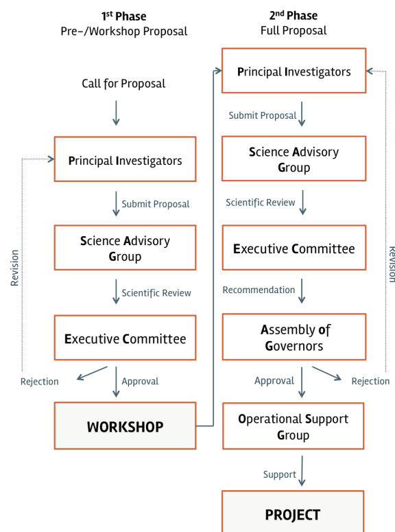
Fig. 11.1: Flow of proposals through ICDP panels
