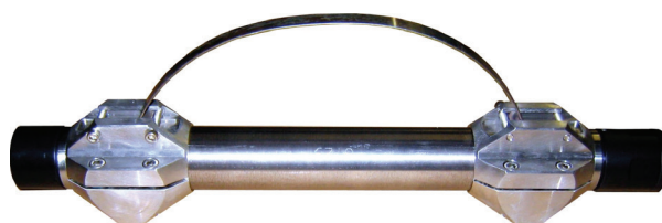
Fig. 7.4: Spring bow de-centralizer hole lock concept (photo: SAFOD project)
