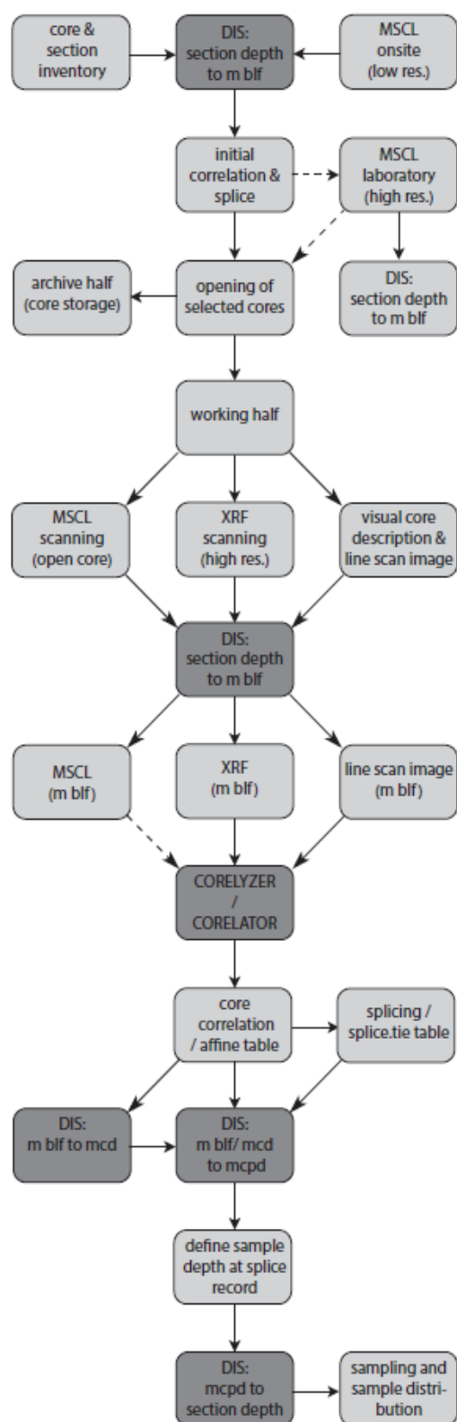
Fig. 2: Schematic workflow for the laboratory work and data management for lake drilling projects ( mblf : meters below lake floor, mcd : meters corrected depth, mcpd : meters composite depth)
